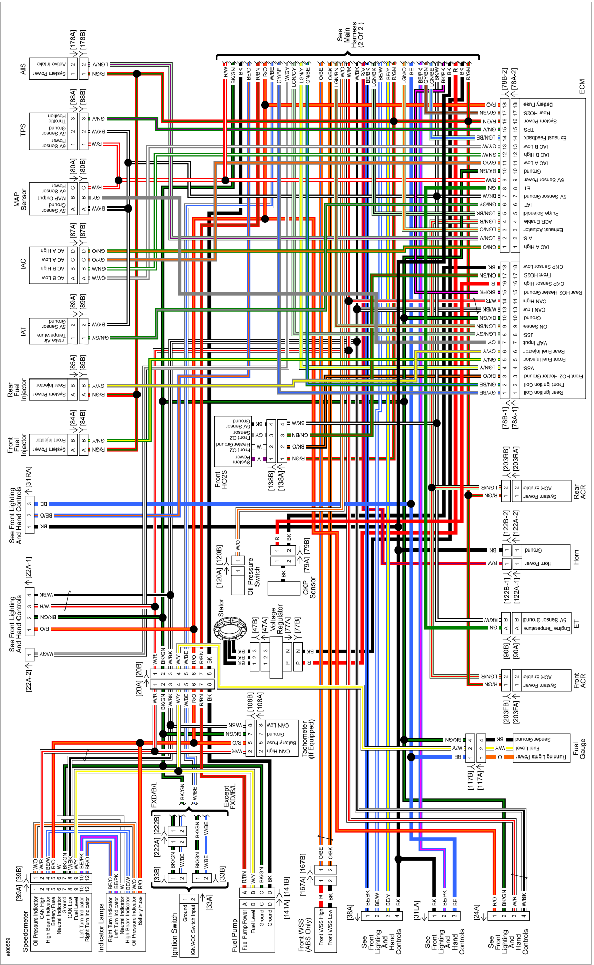
Figure B-10. Main Harness 1 of 2: 2013 Dyna
