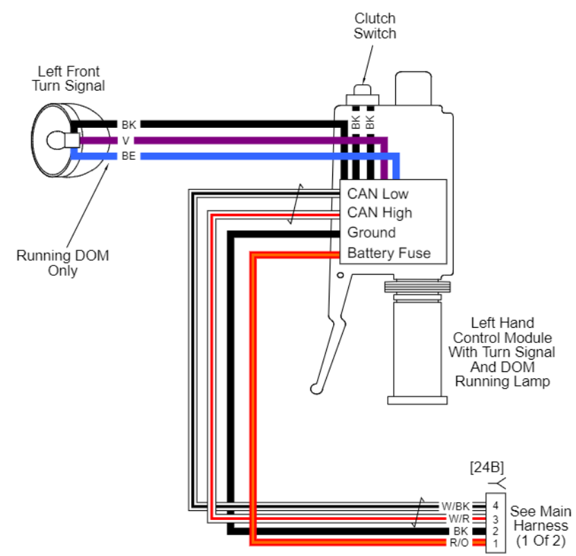
Front Lighting and Hand Controls: 2011 Softail
