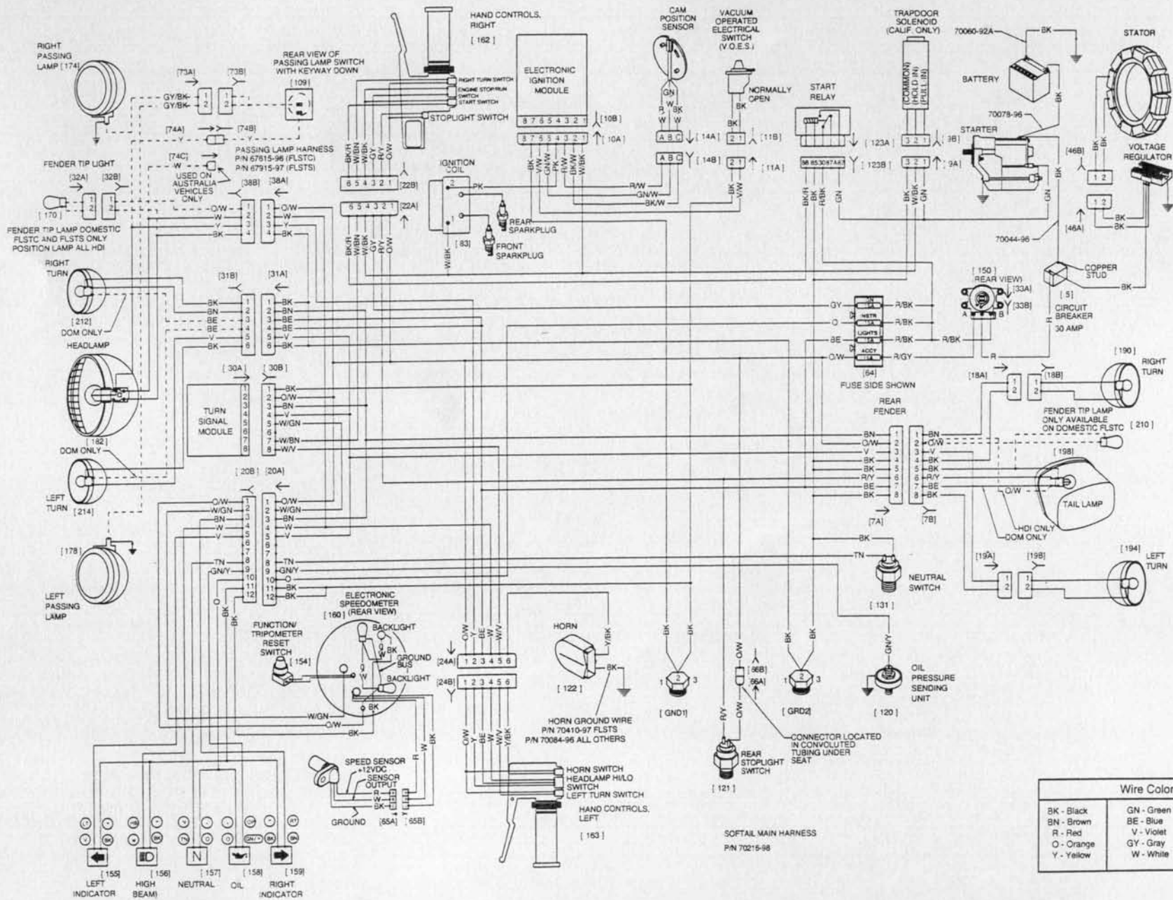
1998 SOFTAIL WIRING DIAGRAM (Domestic and International Models), Main Harness
