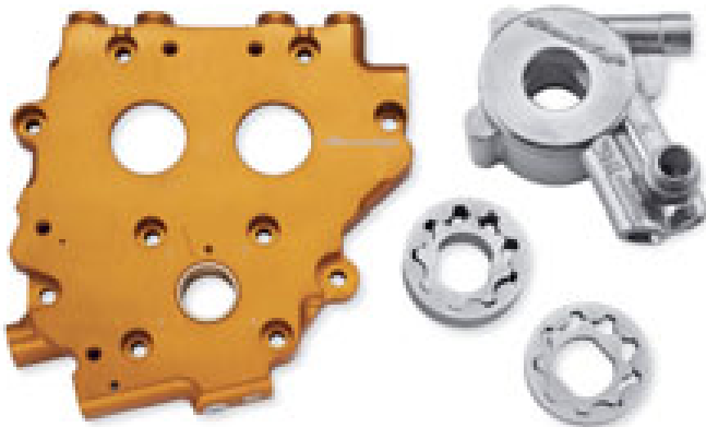
F. SCREAMIN' EAGLE BILLET CAM SUPPORT PLATE WITH HIGH VOLUME OIL PUMP
