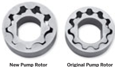
New Pump Rotor
