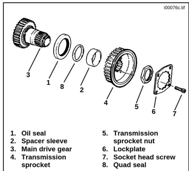
Figure 1. Transmission Sprocket Components
