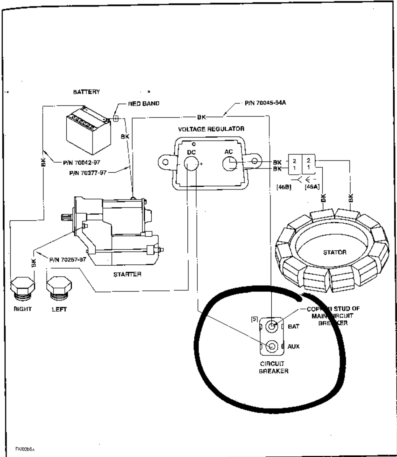
FLHT/C/U, FLTR and FLHR/C Models Charging System Circuit
