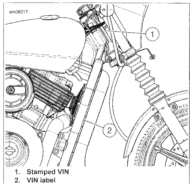
Figure 3-1. VIN Locations
