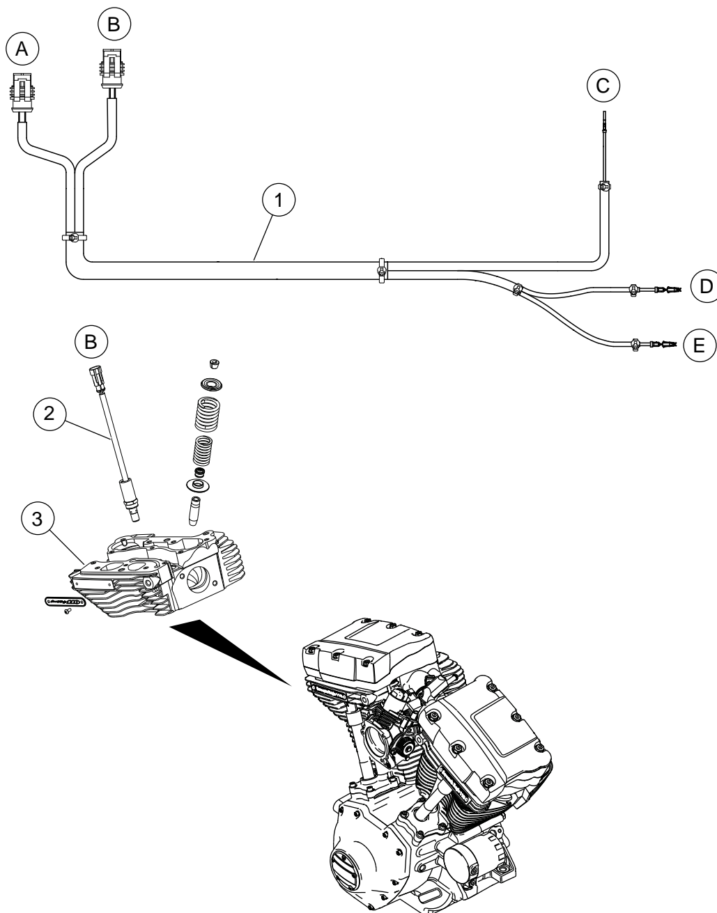
Figure 6. Service Parts: Automatic Compression Release (ACR) Overlay Wire Harness Kit
