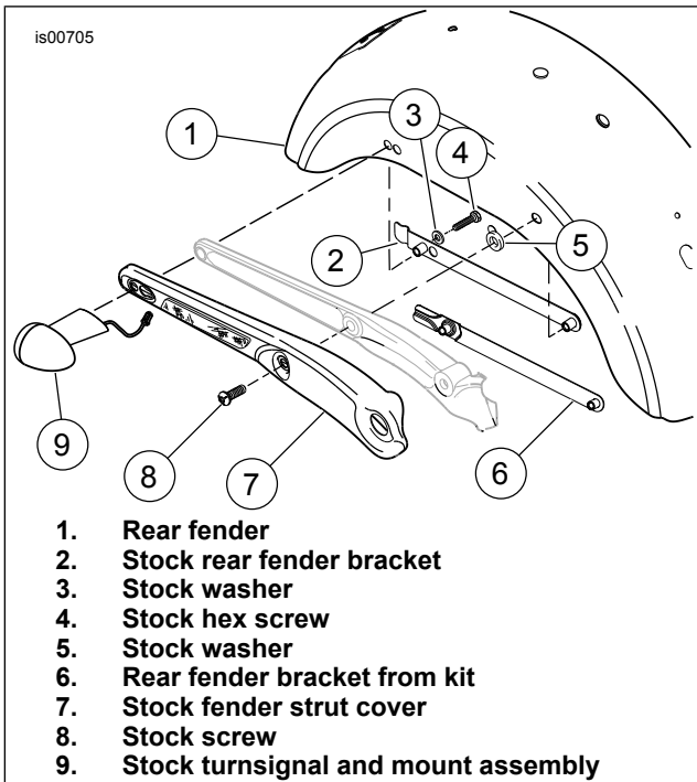
Figure 2. Replace rear fender bracket
