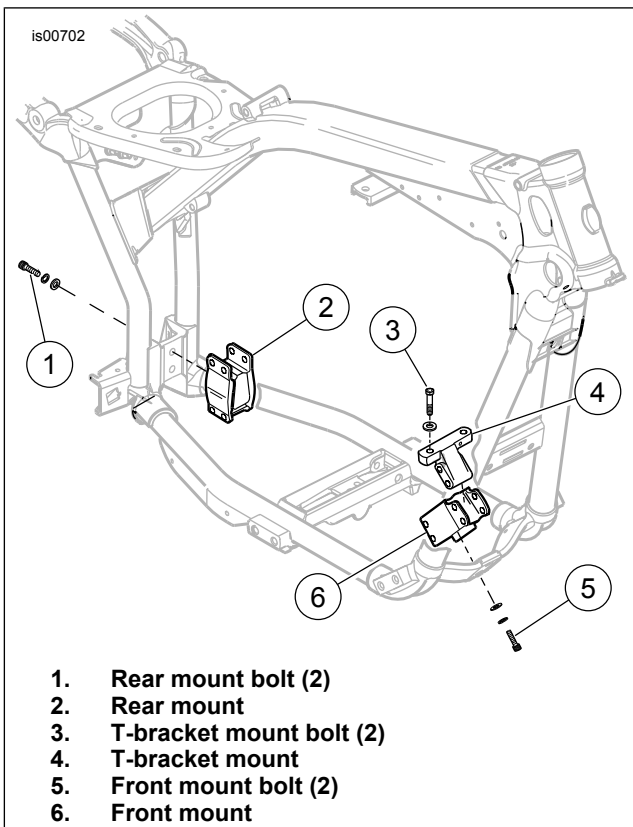
Figure 8. Vehicle Alignment
