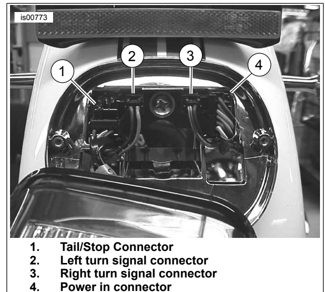
Figure 1. Remove Connectors
